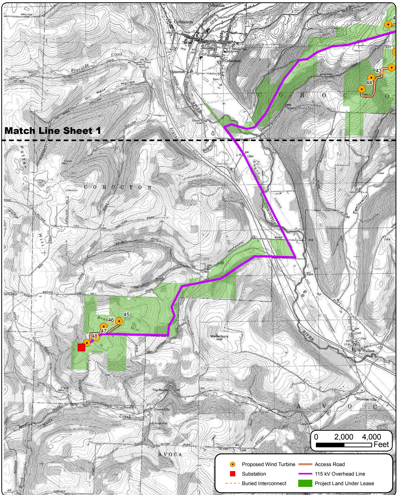
Figure 3: Proposed Project Layout Sheet 2 of 2
