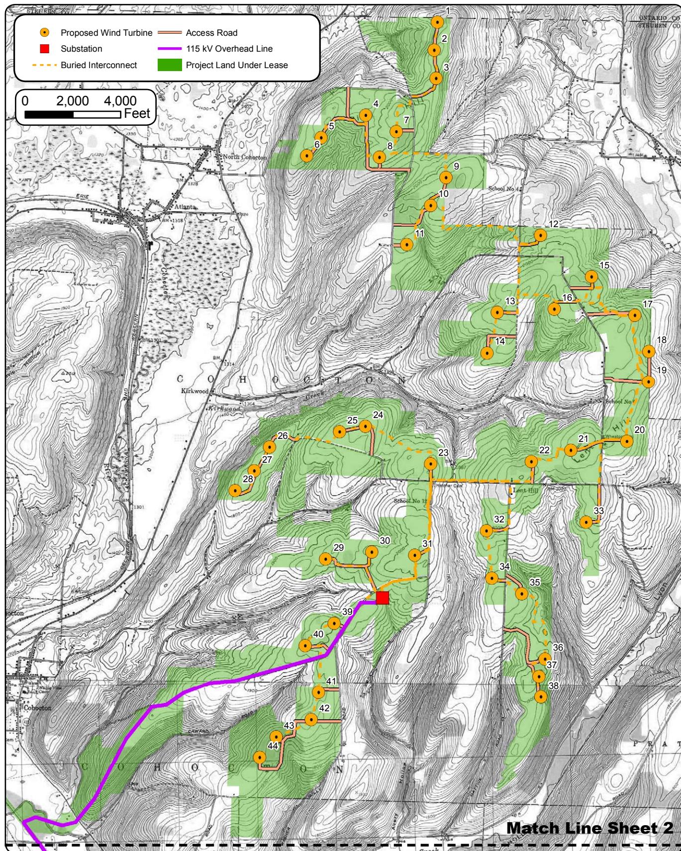
Figure 3: Proposed Project Layout Sheet 1 of 2
